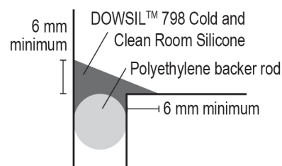
Figure 3: Fillet joint.
