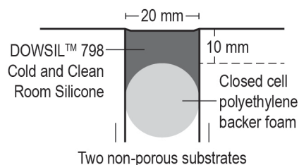
Figure 1: Deep joint.
